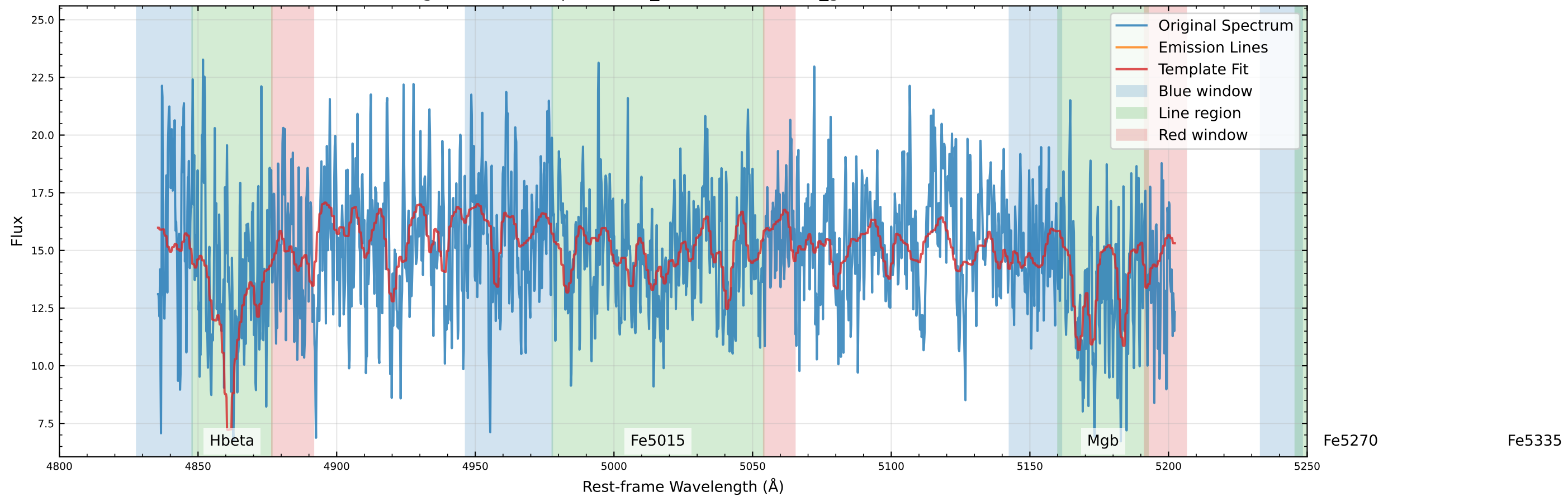
Original Data Comparison (v_star=74.0 km/s, v_gas=26.1 km/s)
