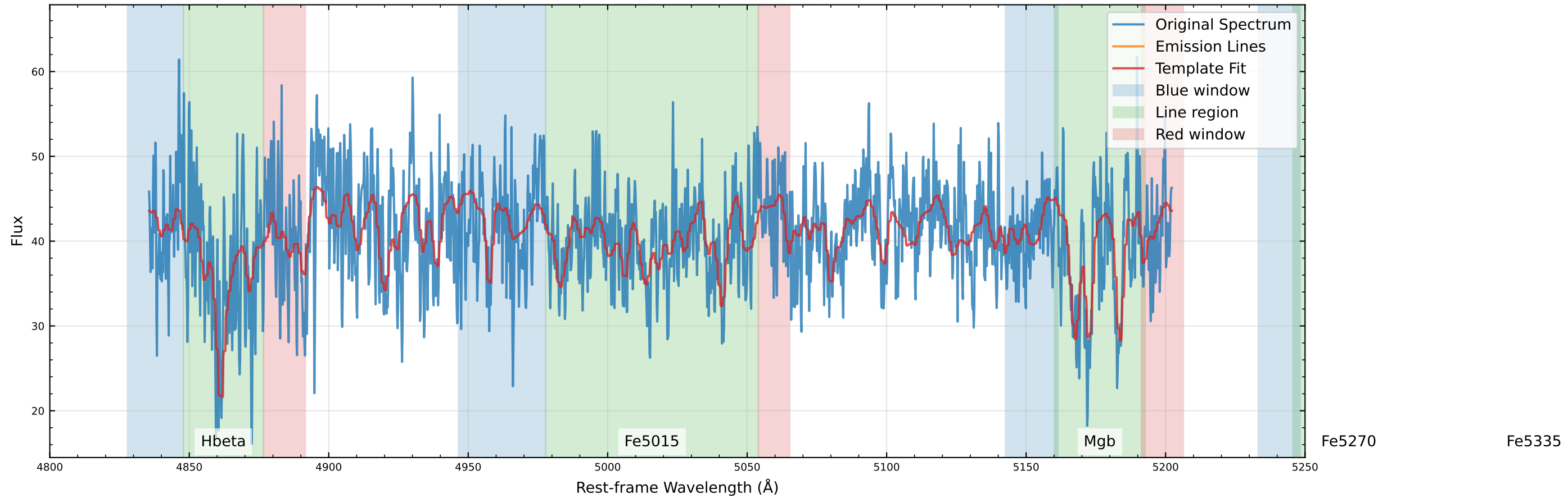
Original Data Comparison (v_star=-14.2 km/s, v_gas=70.1 km/s)
