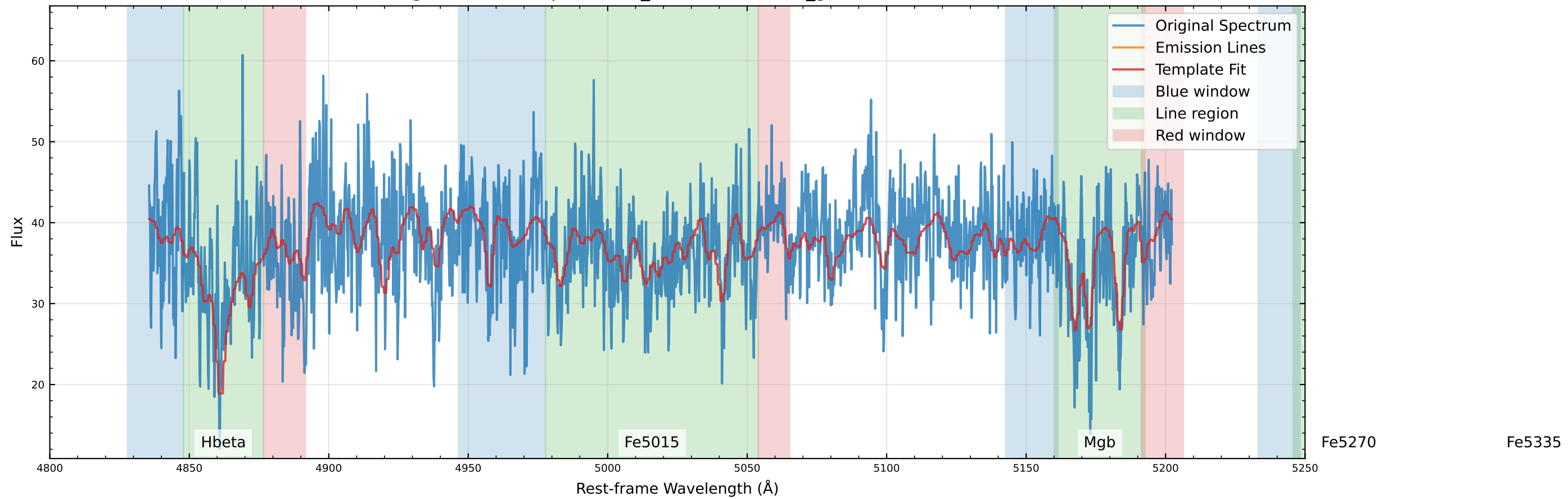
Original Data Comparison (v_star=-2.6 km/s, v_gas=276.5 km/s)
