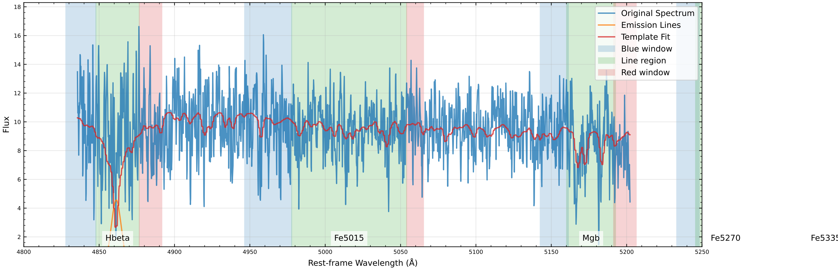
Original Data Comparison (v_star=-30.1 km/s, v_gas=31.1 km/s)
