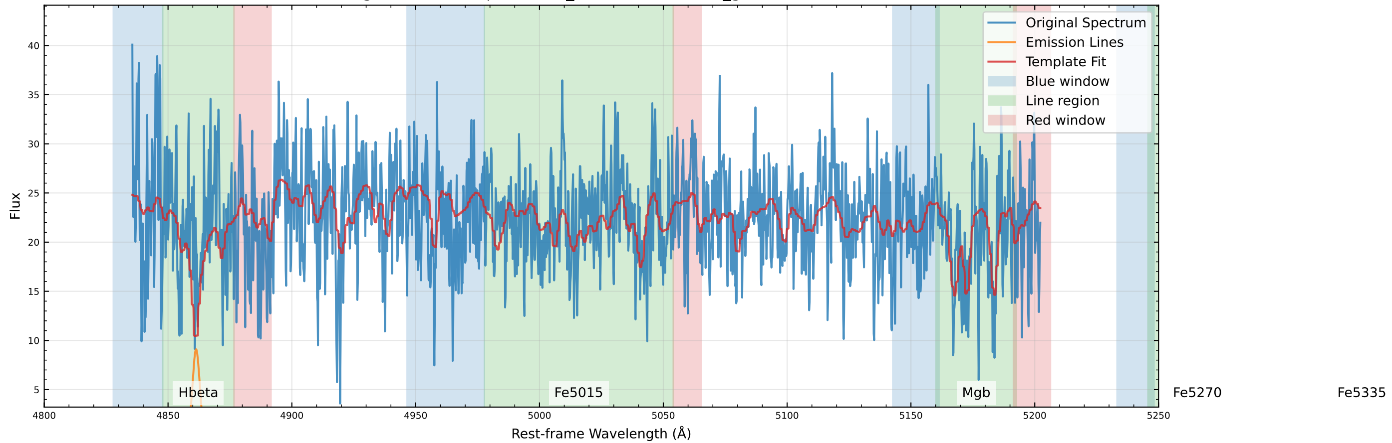
Original Data Comparison (v_star=-15.3 km/s, v_gas=-85.3 km/s)
