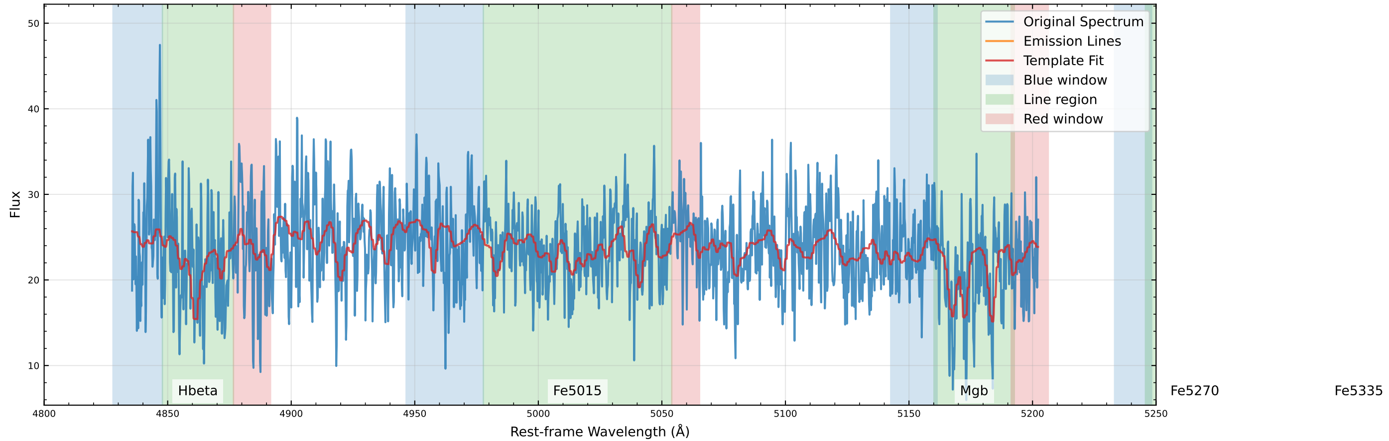
Original Data Comparison (v_star=-6.2 km/s, v_gas=-51.3 km/s)
