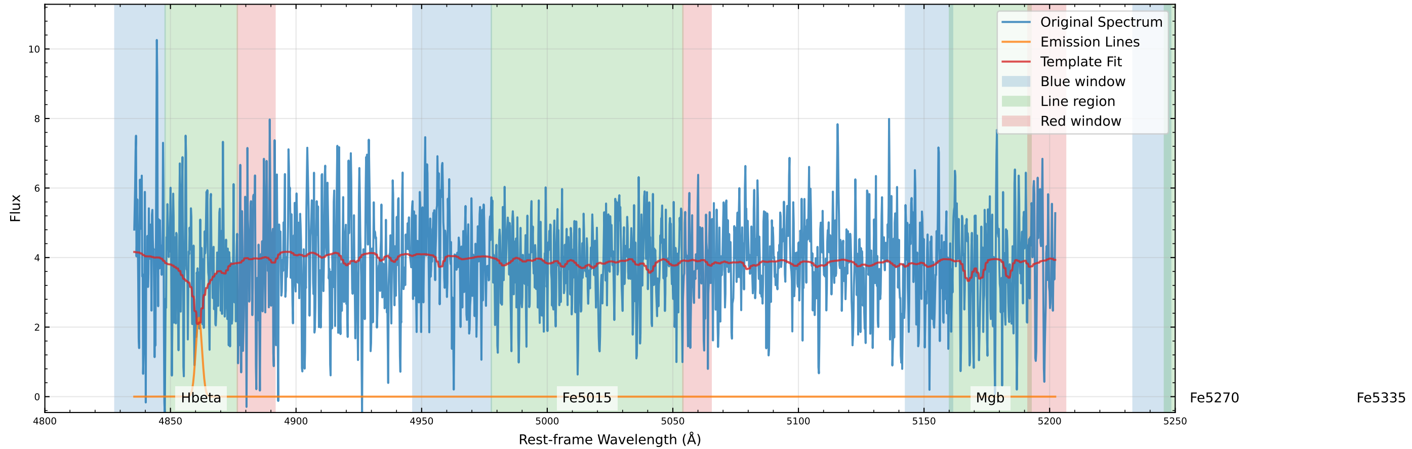
Original Data Comparison (v_star=49.3 km/s, v_gas=170.8 km/s)
