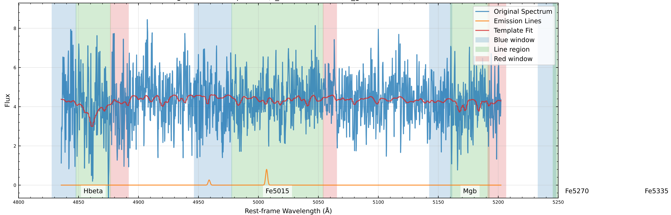
Original Data Comparison (v_star=-18.2 km/s, v_gas=5.0 km/s)
