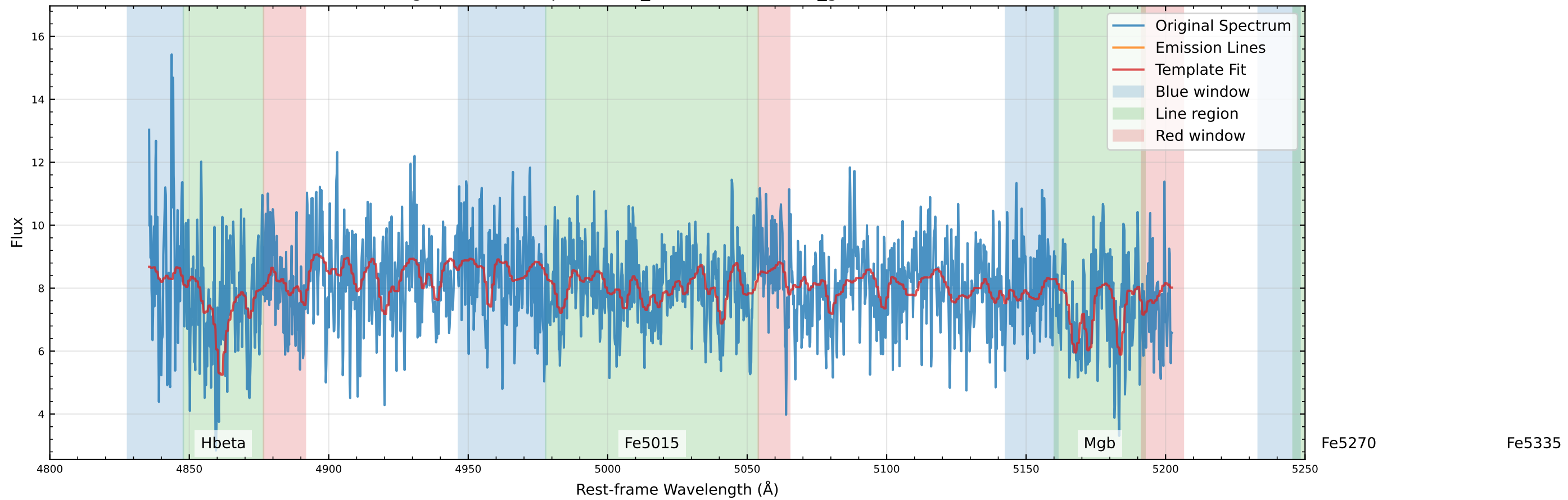
Original Data Comparison (v_star=-49.2 km/s, v_gas=20.6 km/s)
