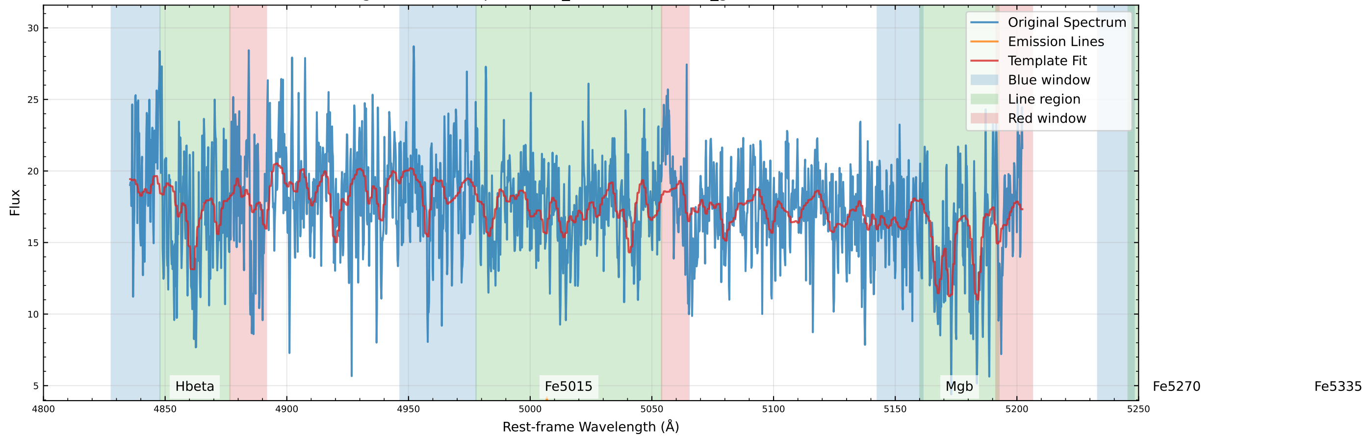
Original Data Comparison (v_star=48.0 km/s, v_gas=23.2 km/s)
