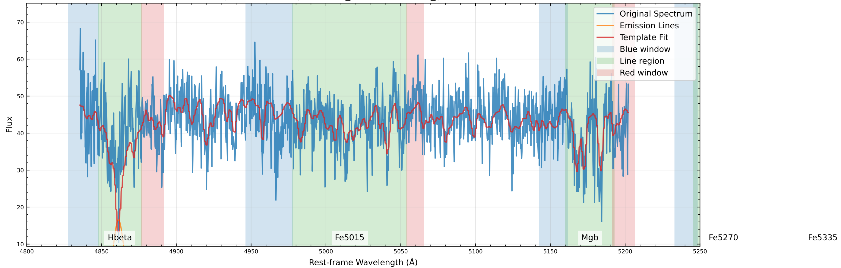
Original Data Comparison (v_star=3.0 km/s, v_gas=129.5 km/s)
