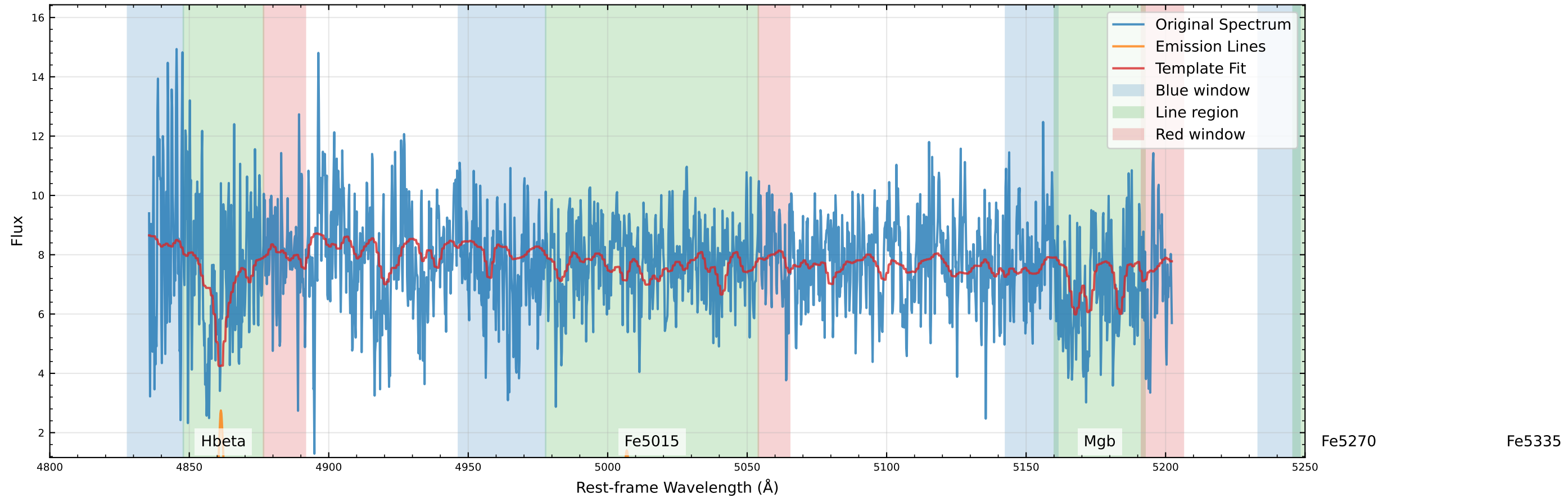
Original Data Comparison (v_star=-107.5 km/s, v_gas=-159.0 km/s)
