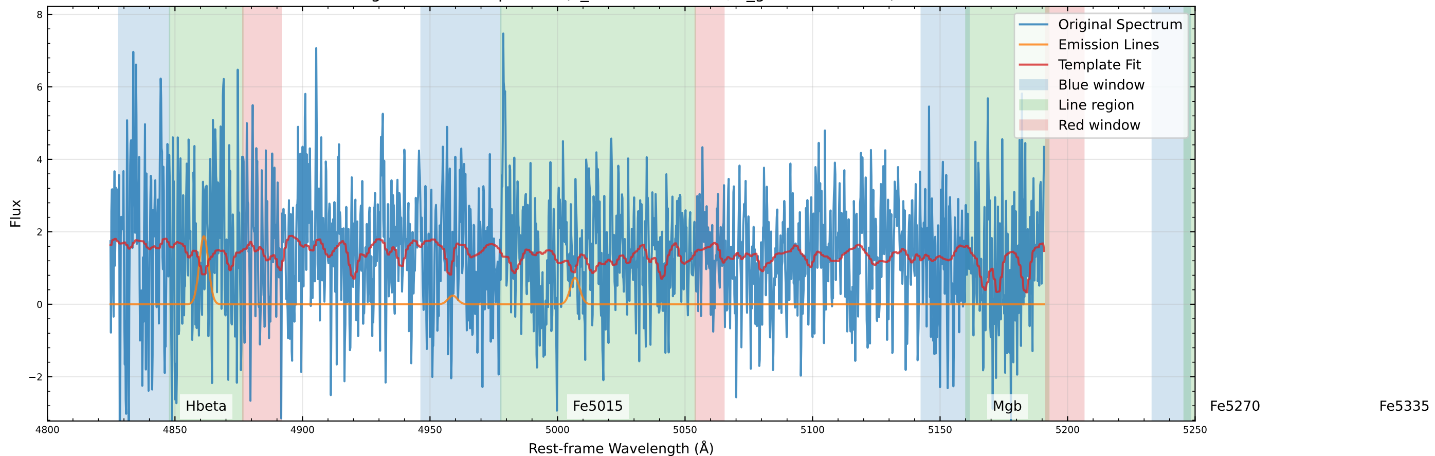
Original Data Comparison (v_star=162.3 km/s, v_gas=358.1 km/s)
