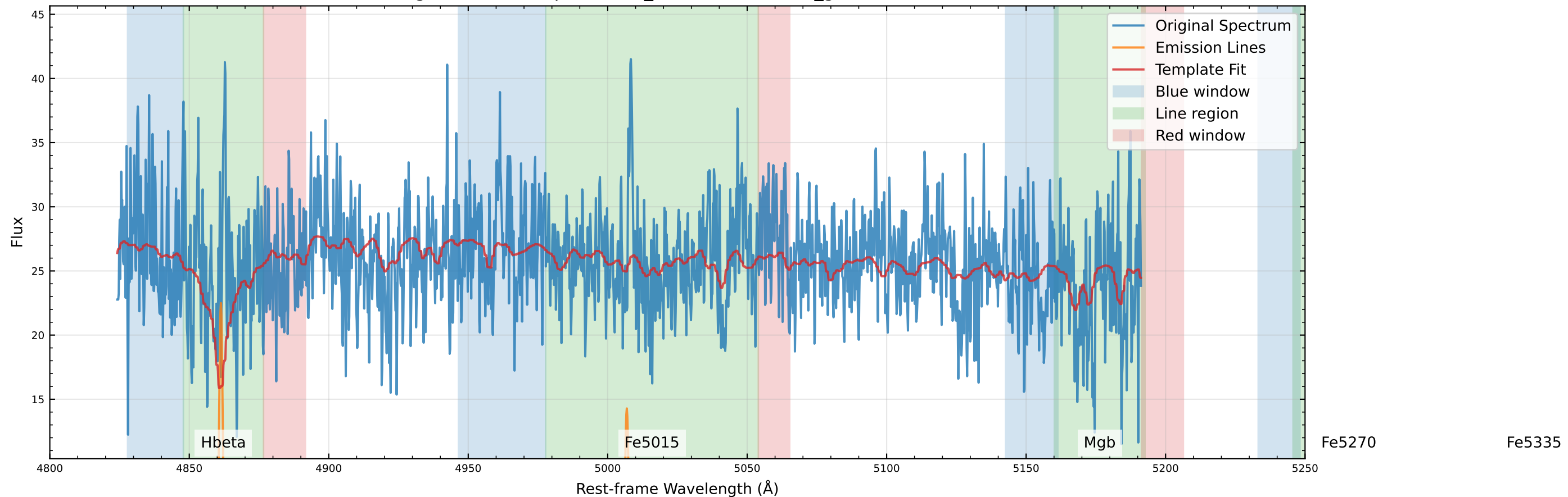
Original Data Comparison (v_star=60.0 km/s, v_gas=78.6 km/s)
