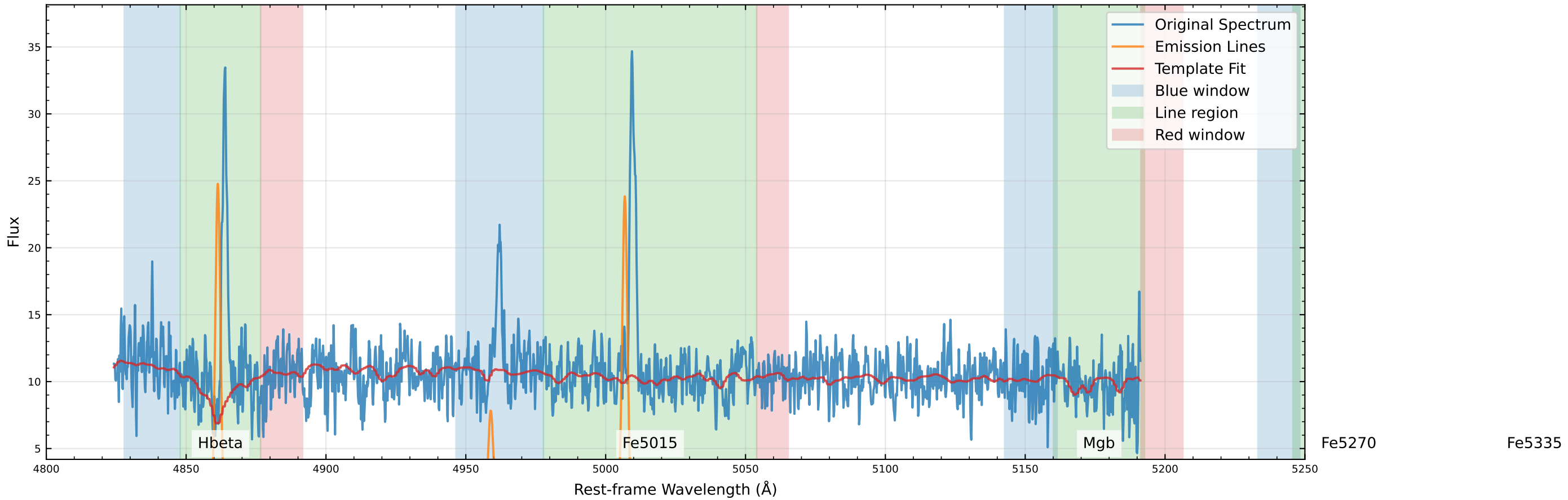
Original Data Comparison (v_star=151.3 km/s, v_gas=160.0 km/s)
