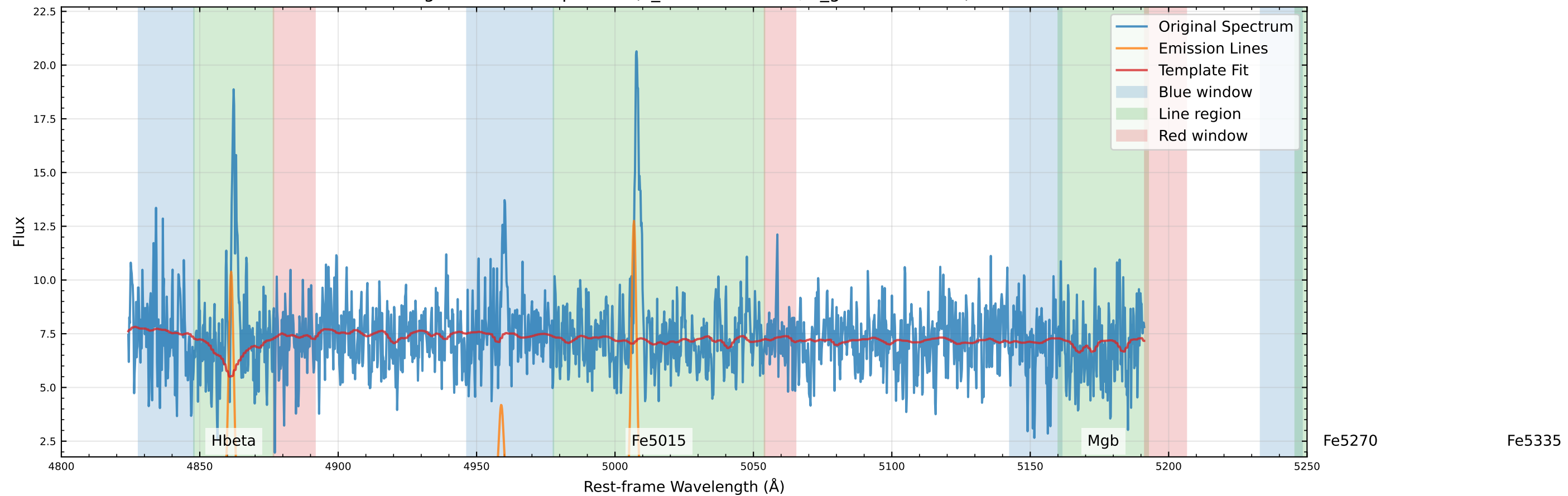
Original Data Comparison (v_star=99.7 km/s, v_gas=71.2 km/s)
