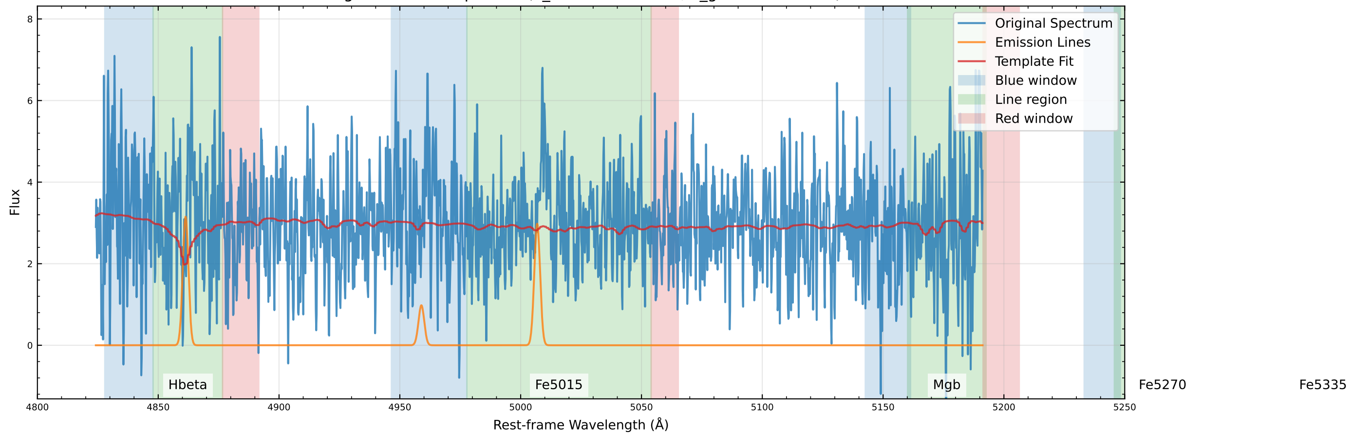
Original Data Comparison (v_star=179.3 km/s, v_gas=145.6 km/s)
