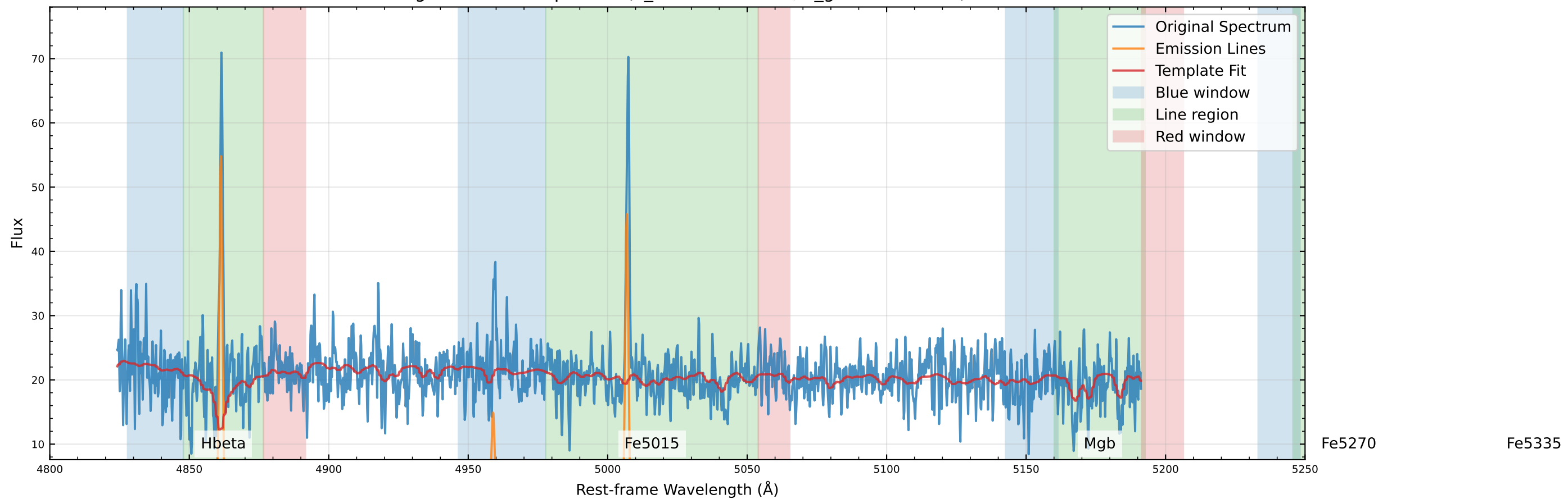
Original Data Comparison (v_star=14.0 km/s, v_gas=17.4 km/s)
