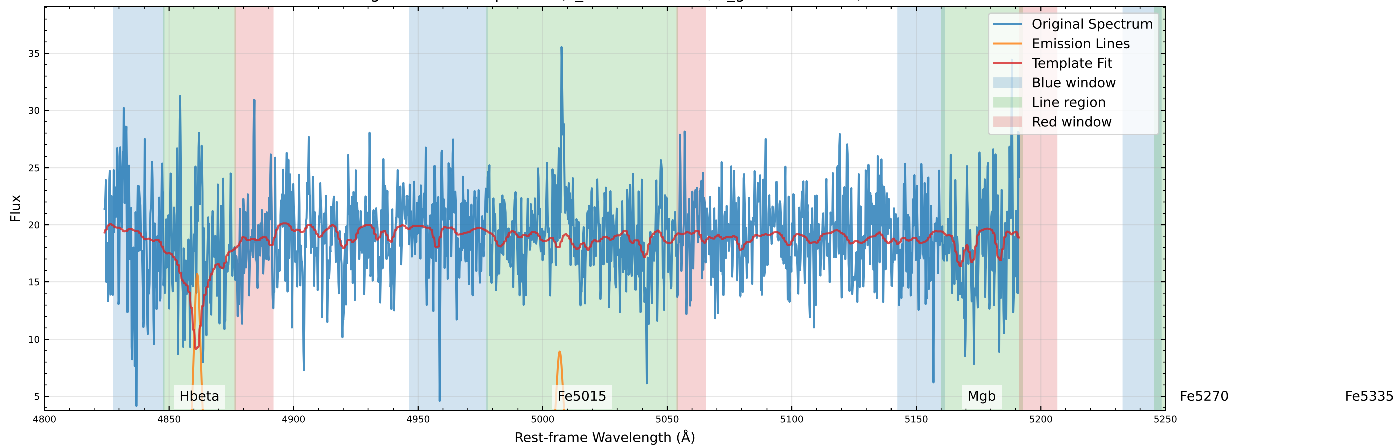
Original Data Comparison (v_star=43.0 km/s, v_gas=45.8 km/s)
