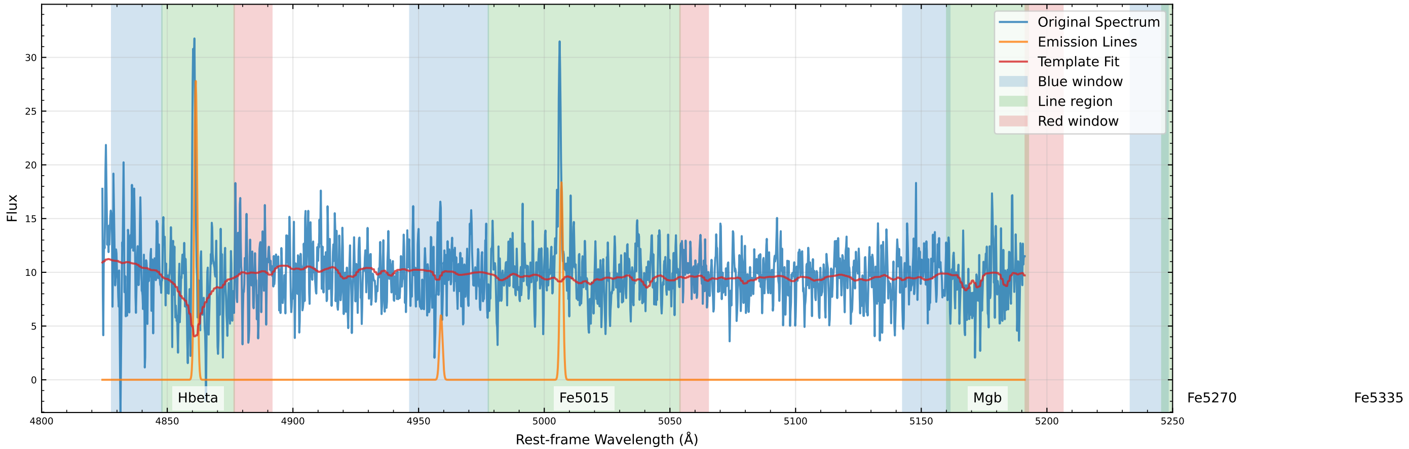
Original Data Comparison (v_star=-33.4 km/s, v_gas=-45.9 km/s)
