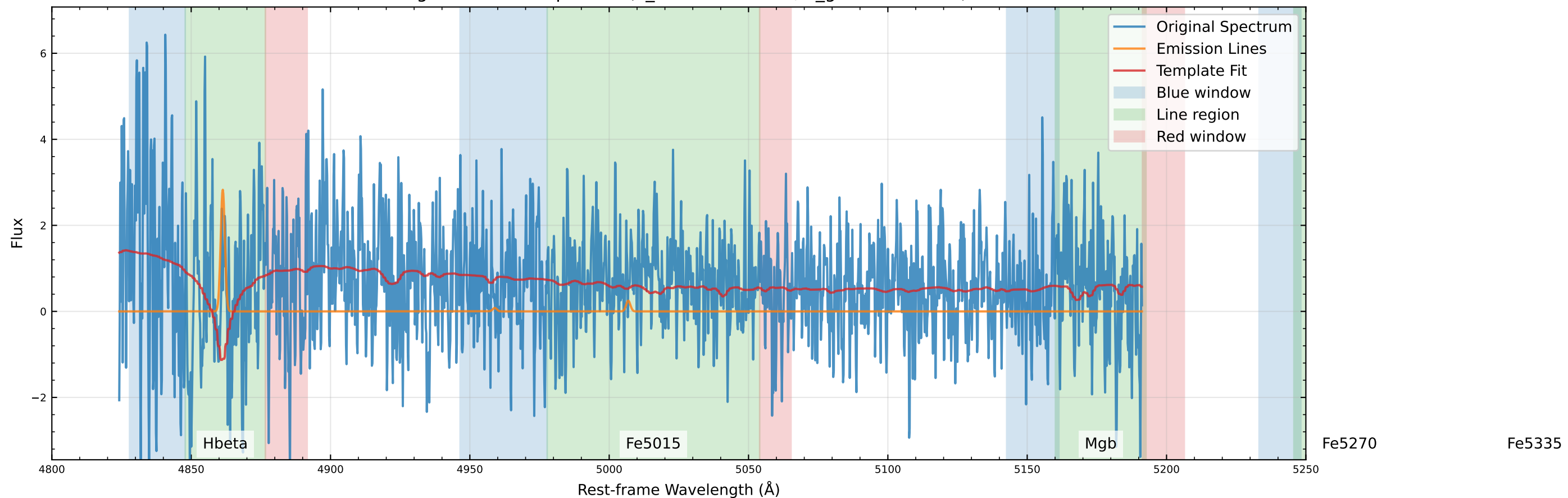
Original Data Comparison (v_star=15.6 km/s, v_gas=22.7 km/s)
