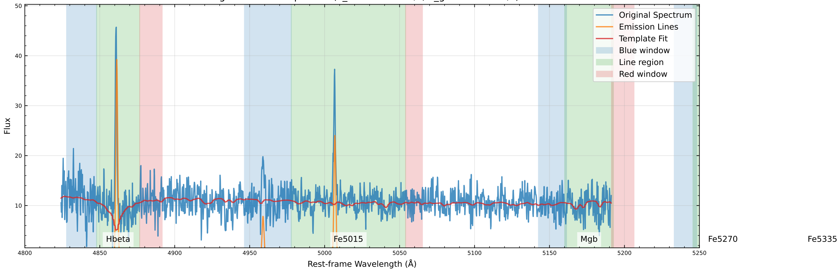
Original Data Comparison (v_star=12.8 km/s, v_gas=-24.8 km/s)
