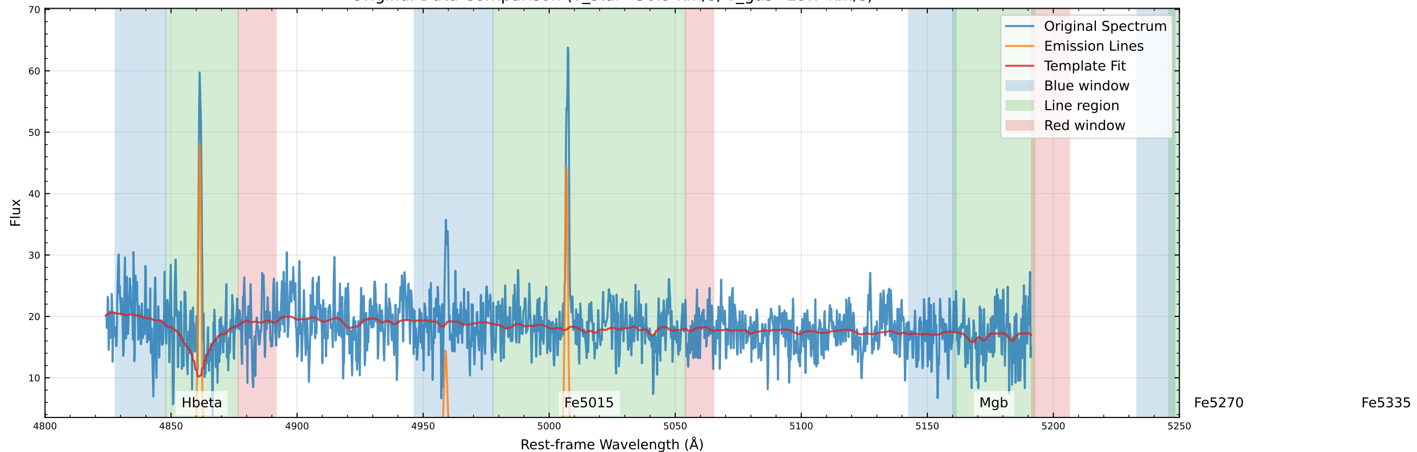
Original Data Comparison (v_star=30.9 km/s, v_gas=19.7 km/s)
