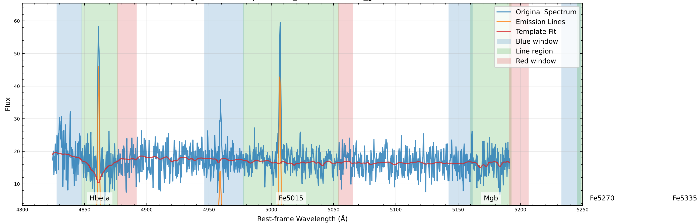
Original Data Comparison (v_star=8.8 km/s, v_gas=3.2 km/s)
