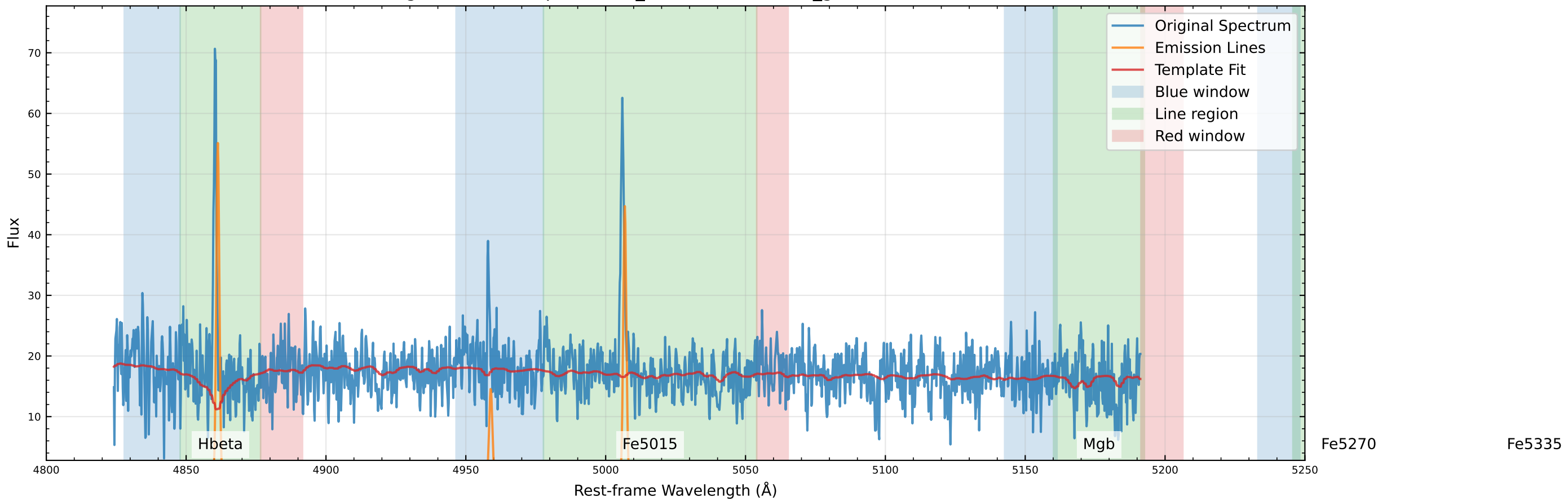
Original Data Comparison (v_star=-35.6 km/s, v_gas=-57.0 km/s)
