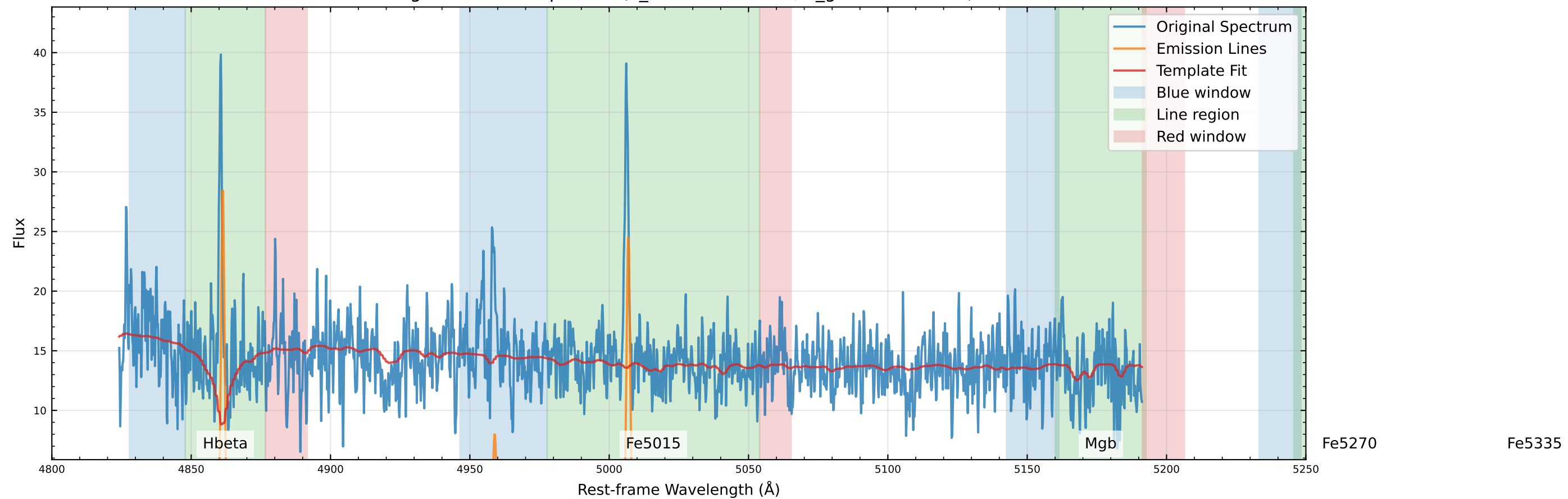
Original Data Comparison (v_star=-36.9 km/s, v_gas=-43.7 km/s)
