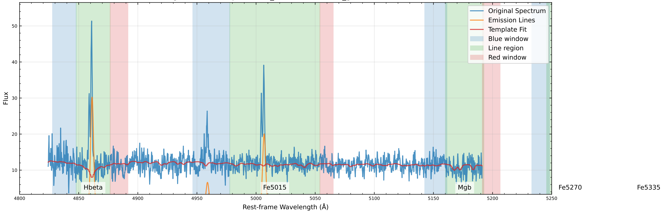
Original Data Comparison (v_star=16.4 km/s, v_gas=-44.7 km/s)
