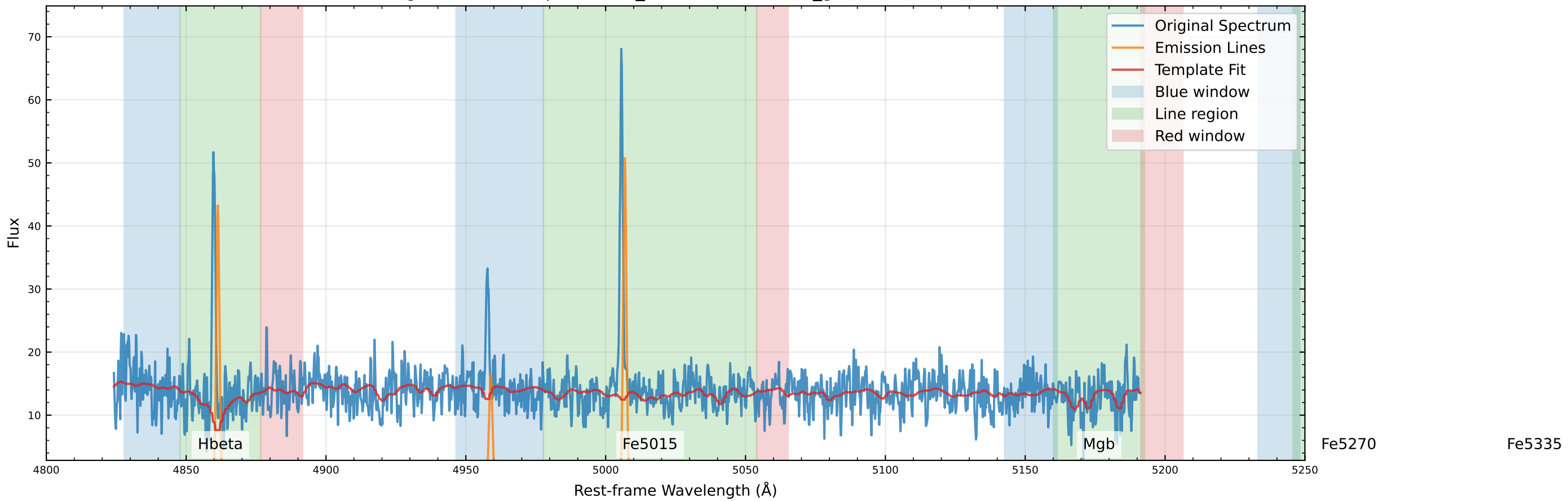
Original Data Comparison (v_star=-65.5 km/s, v_gas=-78.8 km/s)
