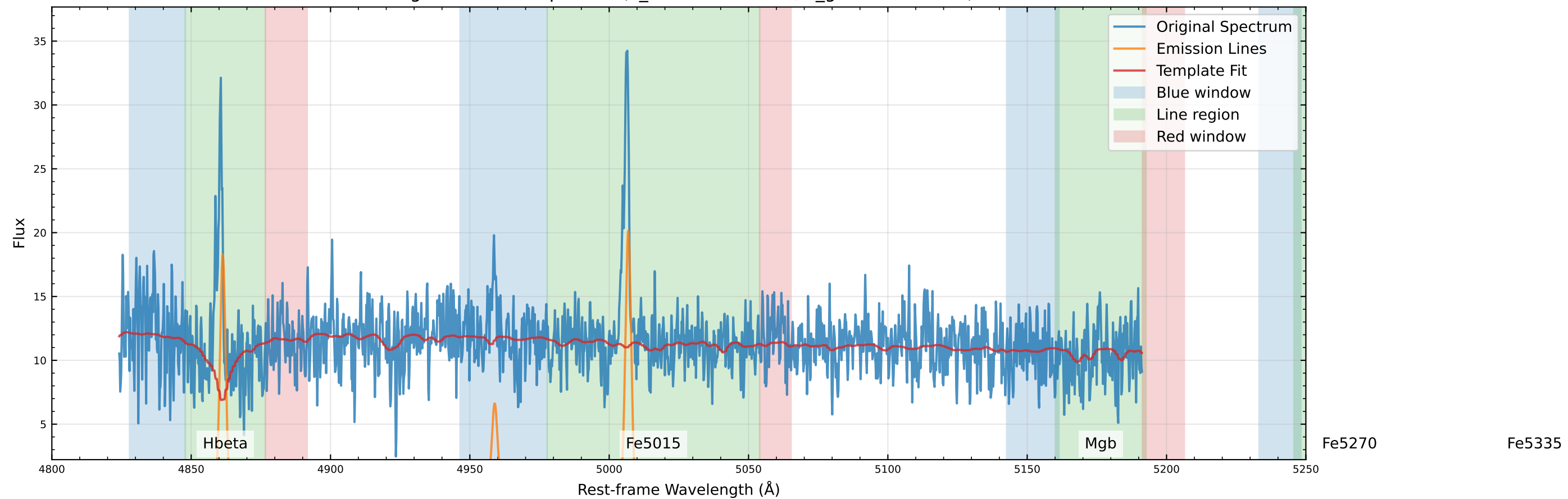
Original Data Comparison ( v_{\text{star}}=-49.9 km/s, v_{\text{gas}}=-50.5 km/s)
