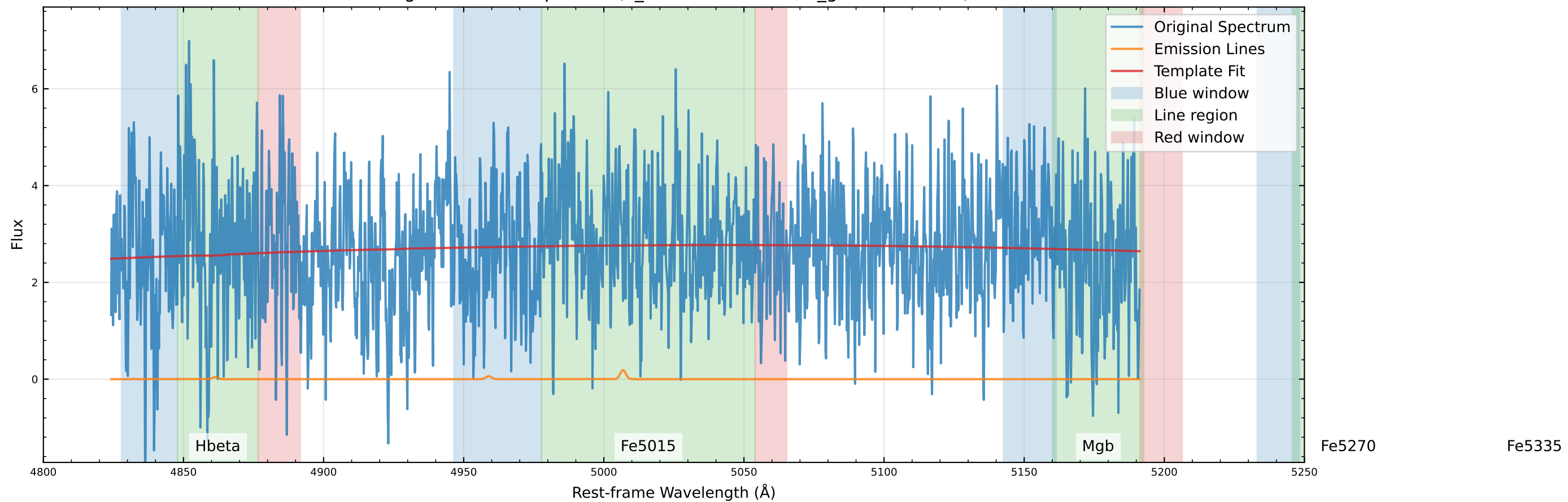
Original Data Comparison (v_star=113.9 km/s, v_gas=99.3 km/s)
