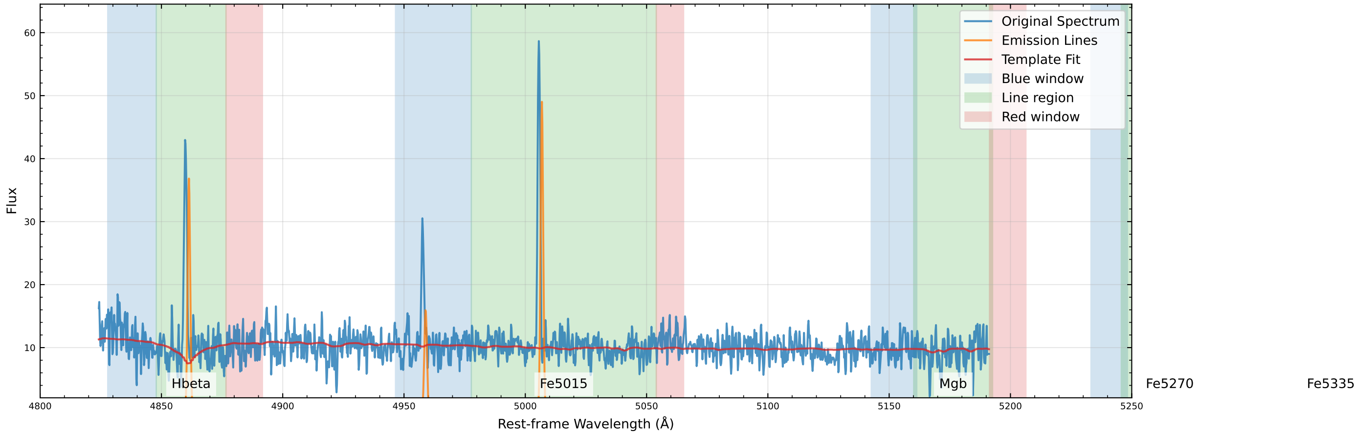
Original Data Comparison (v_star=-93.3 km/s, v_gas=-78.1 km/s)
