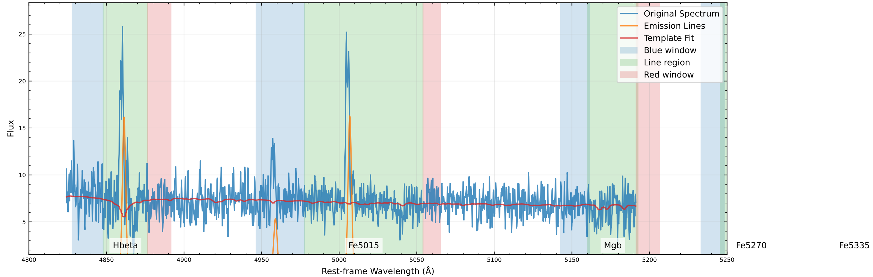
Original Data Comparison (v_star=-204.7 km/s, v_gas=-92.8 km/s)
