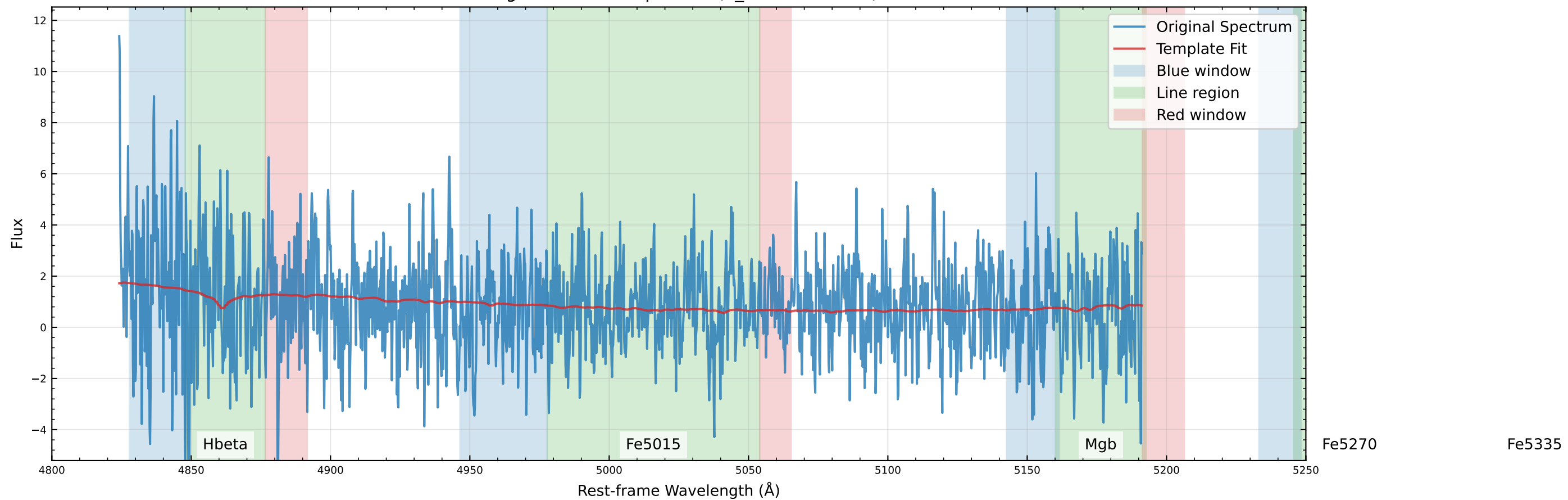
Original Data Comparison (v_star=7.1 km/s)
