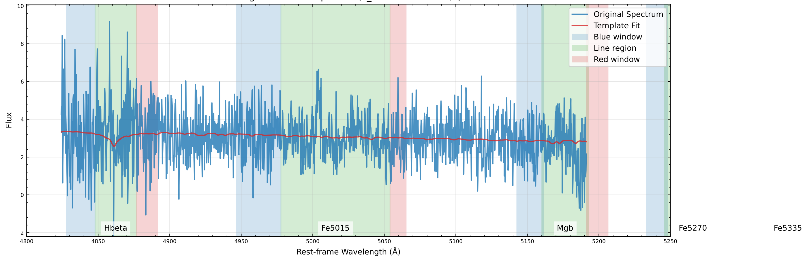
Original Data Comparison (v_star=-1530.9 km/s)
