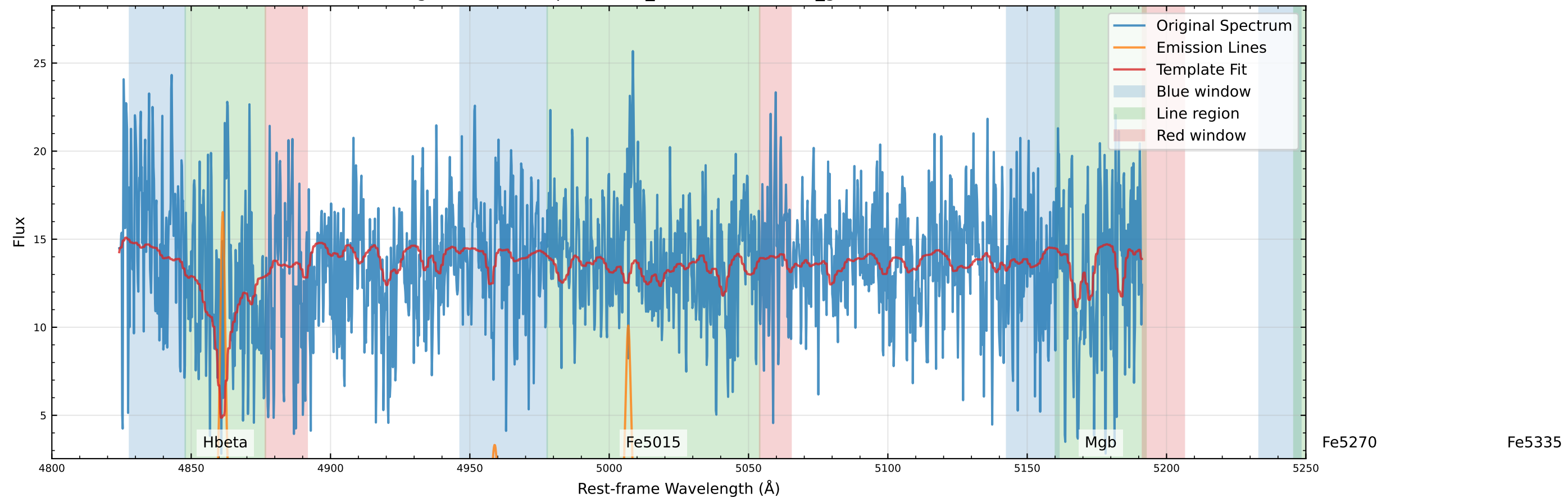
Original Data Comparison (v_star=87.3 km/s, v_gas=85.7 km/s)
