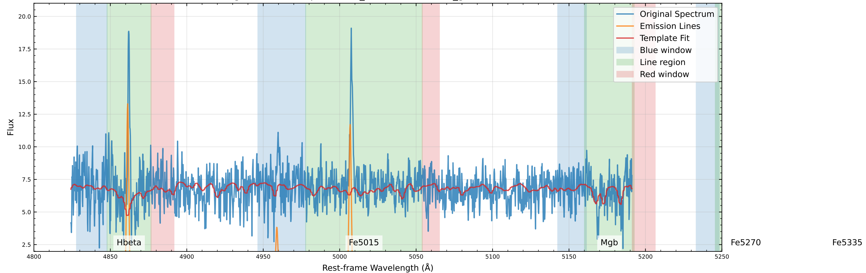
Original Data Comparison (v_star=50.1 km/s, v_gas=49.0 km/s)
