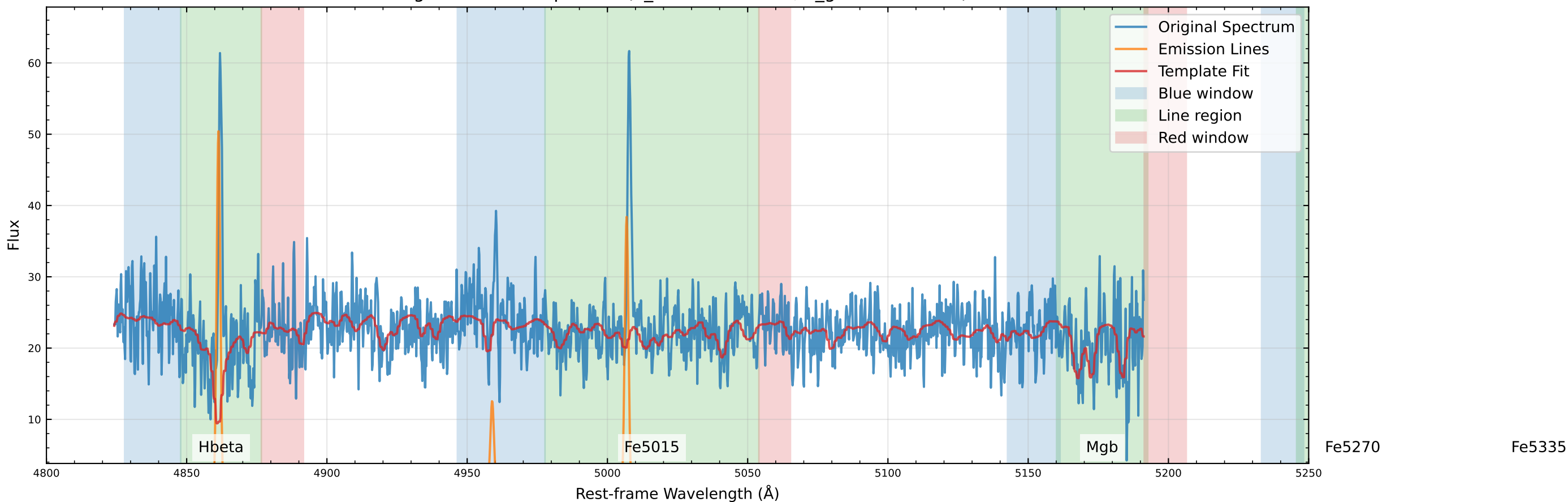
Original Data Comparison (v_star=45.2 km/s, v_gas=50.0 km/s)
