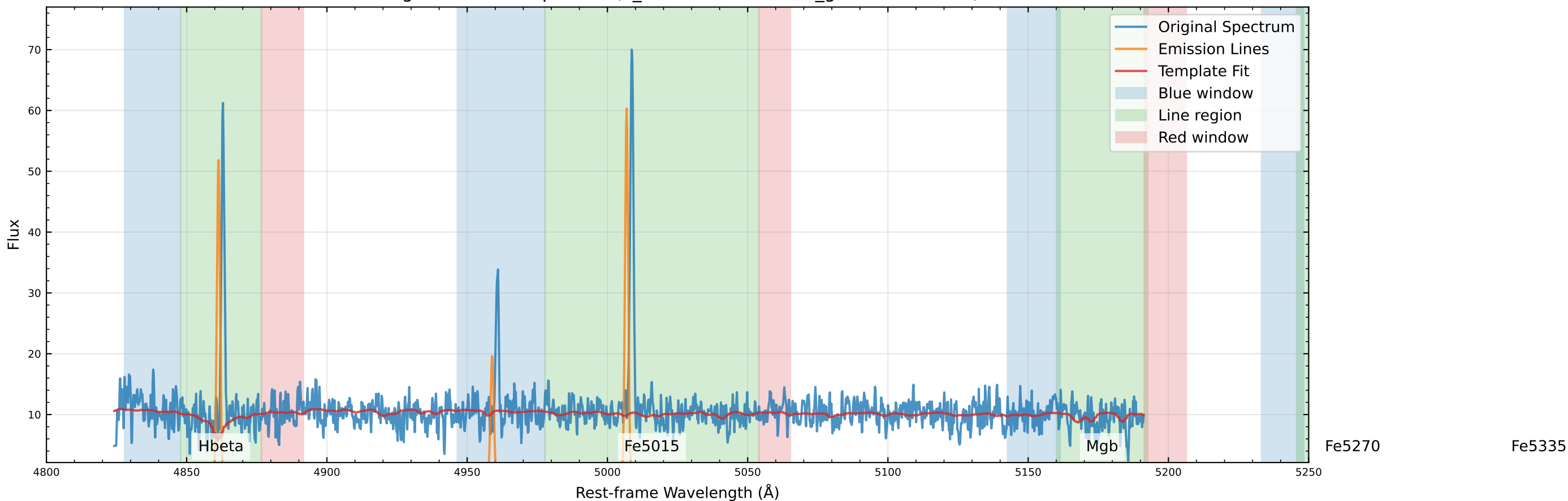
Original Data Comparison (v_star=111.6 km/s, v_gas=105.9 km/s)
