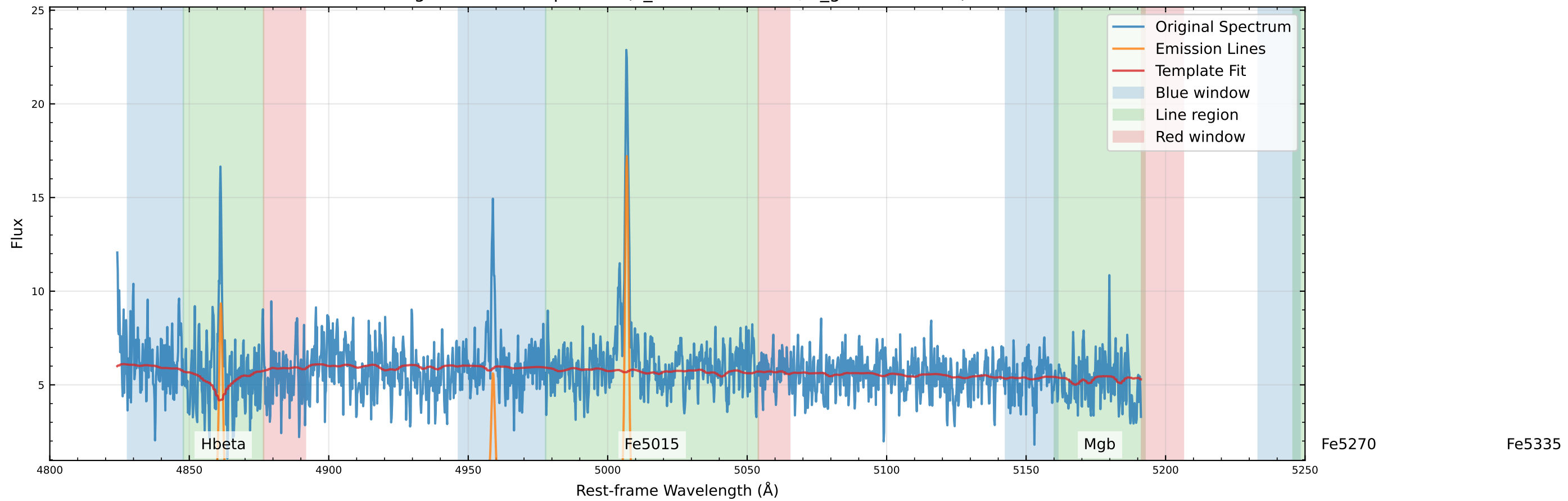
Original Data Comparison (v_star=-41.2 km/s, v_gas=-2.9 km/s)
