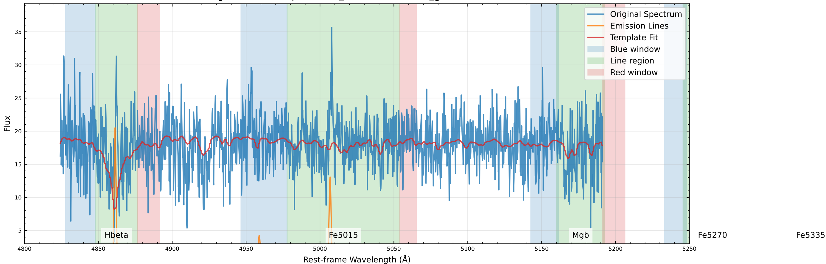
Original Data Comparison (v_star=21.4 km/s, v_gas=55.9 km/s)
