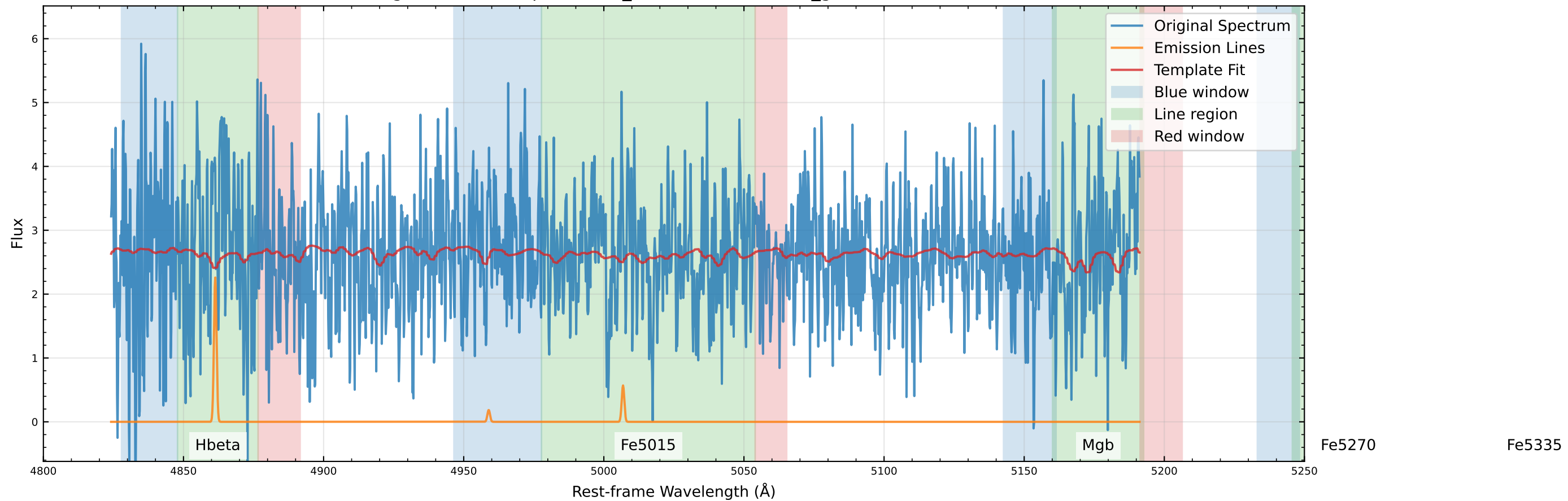
Original Data Comparison (v_star=-466.2 km/s, v_gas=-398.4 km/s)
