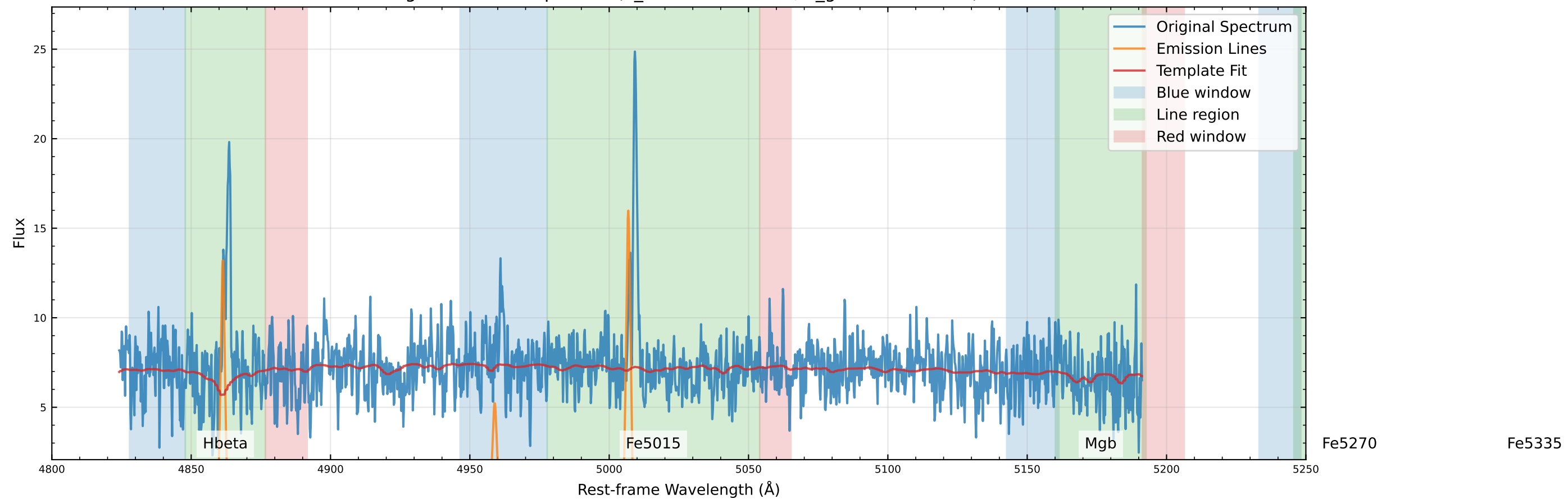
Original Data Comparison (v_star=142.7 km/s, v_gas=140.3 km/s)
