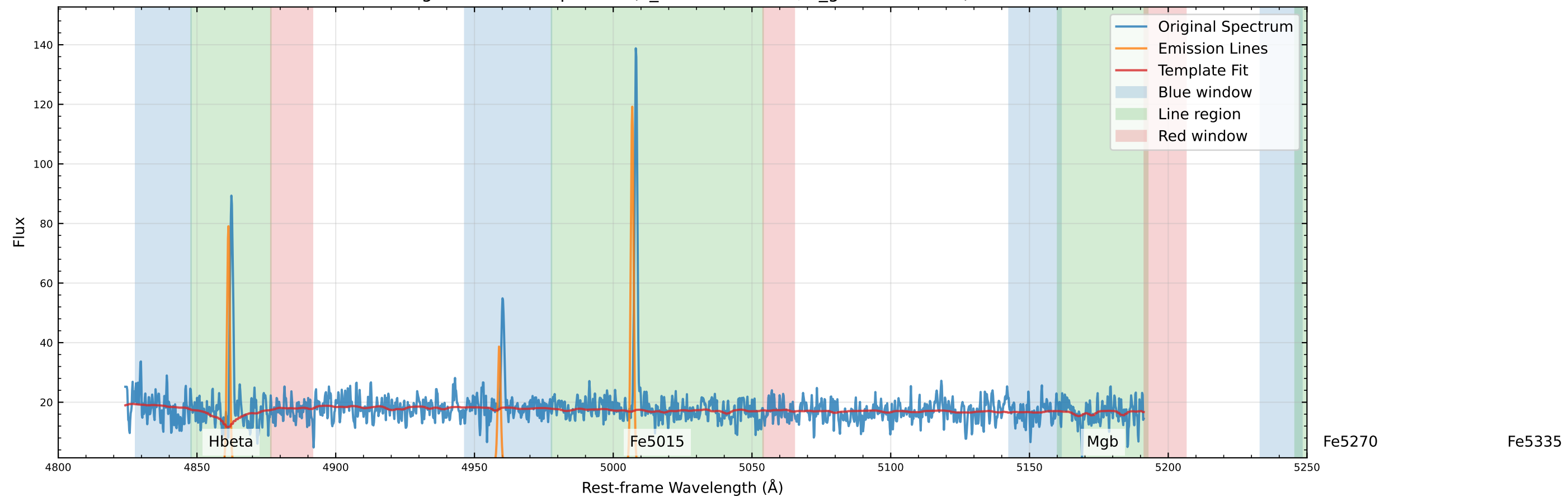
Original Data Comparison (v_star=82.4 km/s, v_gas=77.3 km/s)
