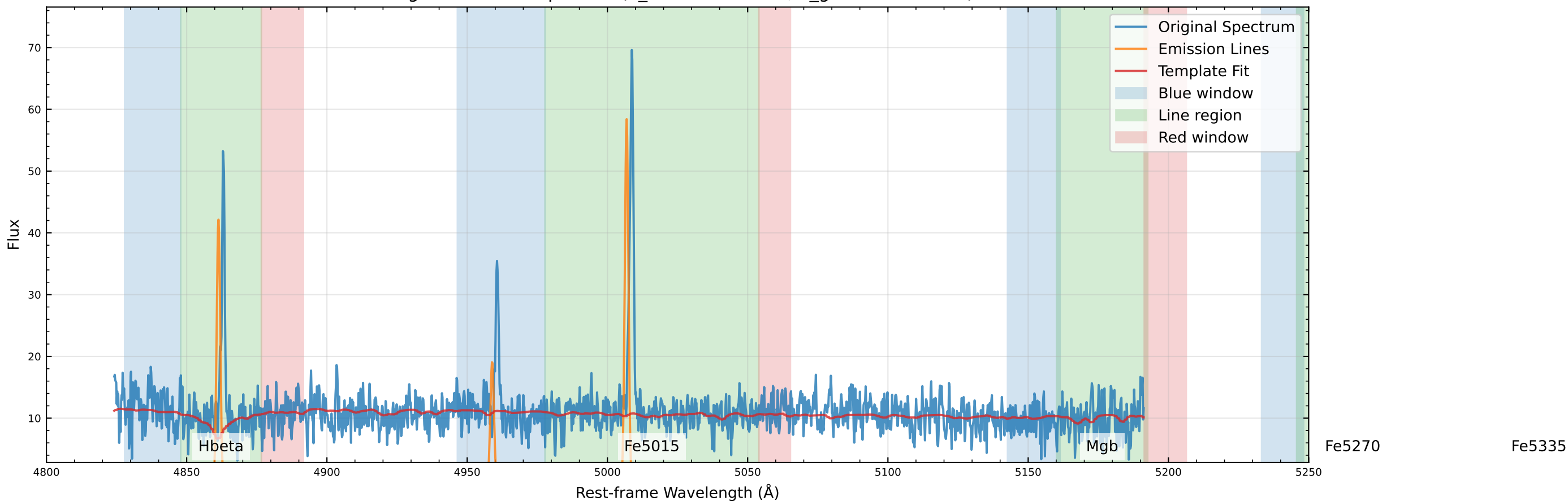
Original Data Comparison (v_star=86.2 km/s, v_gas=106.7 km/s)
