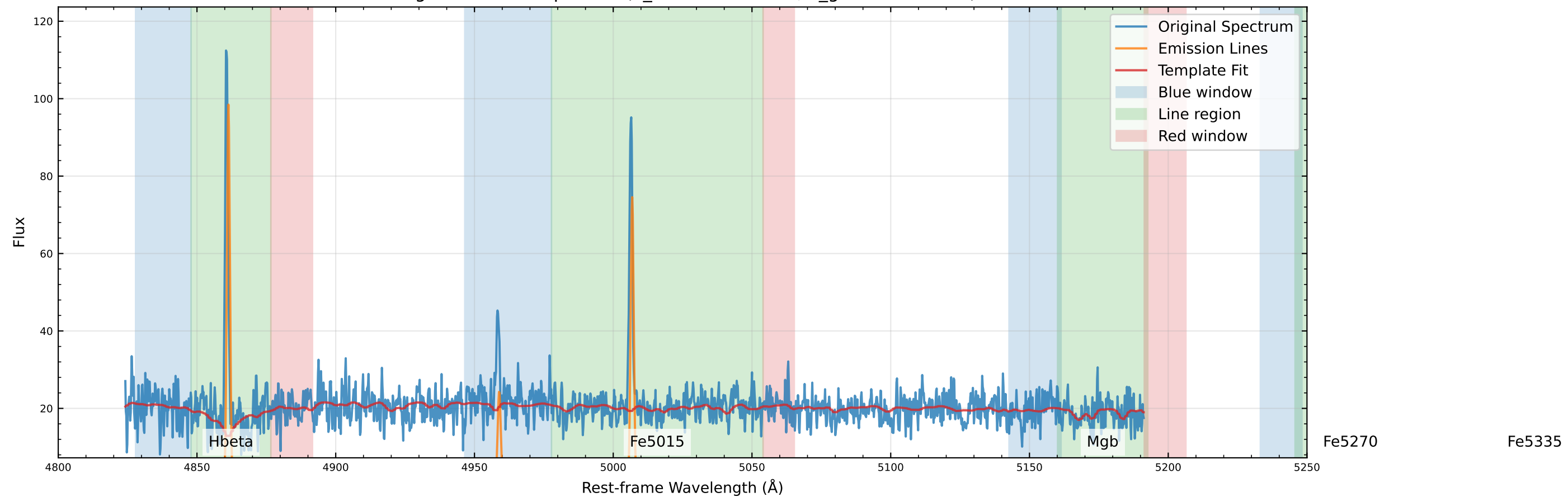
Original Data Comparison (v_star=-18.3 km/s, v_gas=-35.9 km/s)
