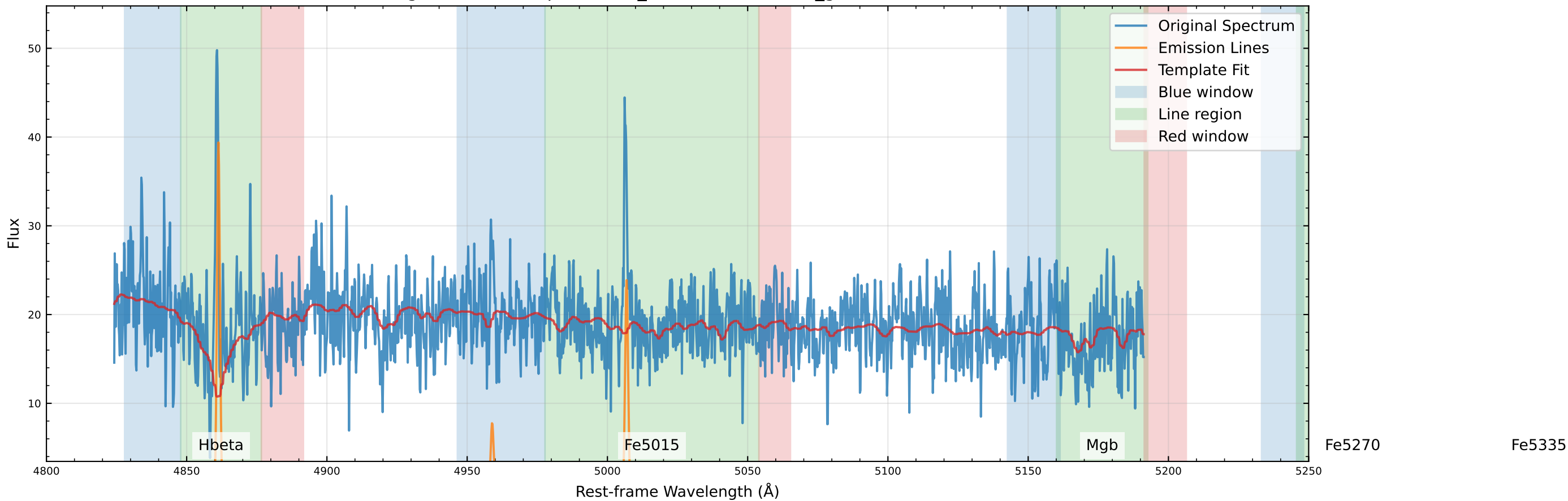
Original Data Comparison (v_star=-24.1 km/s, v_gas=-31.6 km/s)
