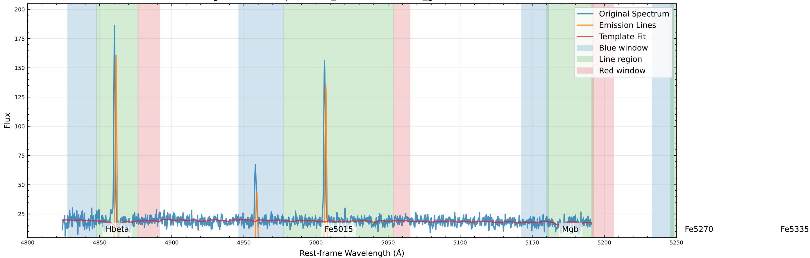
Original Data Comparison (v_star=-47.4 km/s, v_gas=-58.8 km/s)
