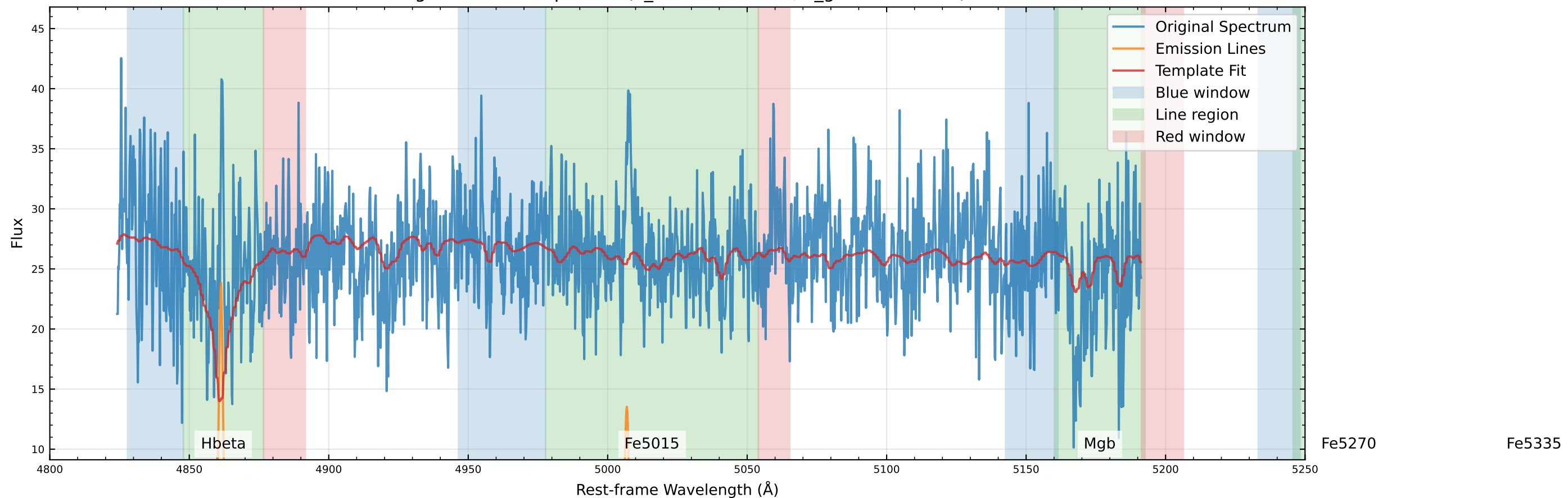
Original Data Comparison (v_star=22.7 km/s, v_gas=23.7 km/s)
