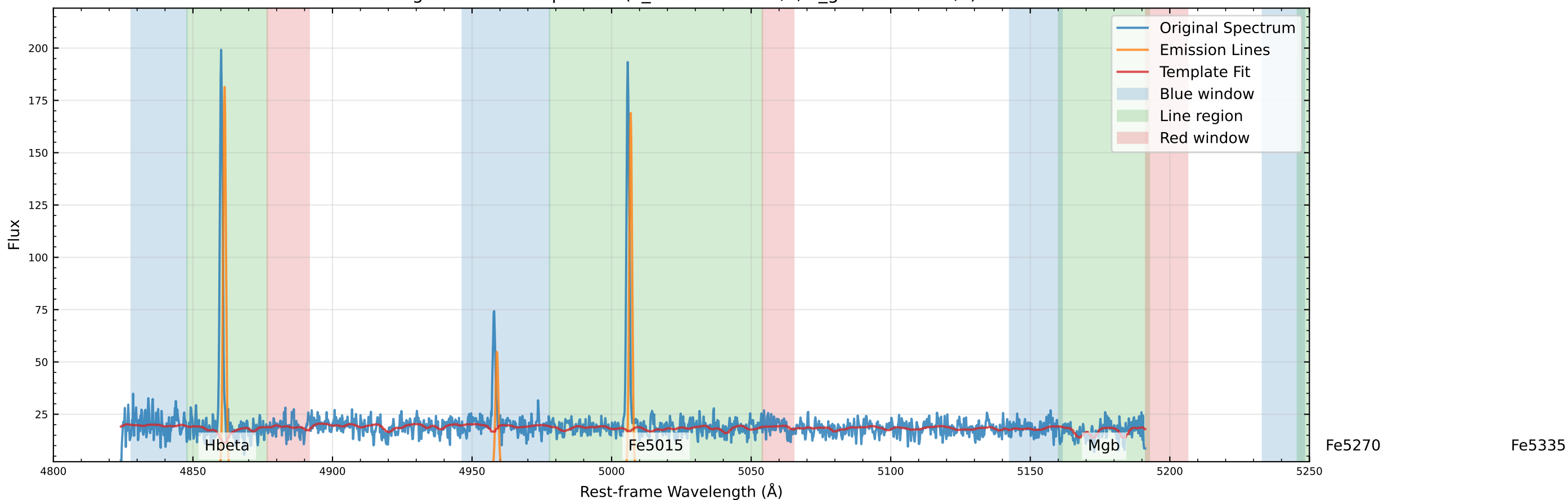
Original Data Comparison (v_star=-65.5 km/s, v_gas=-67.1 km/s)
