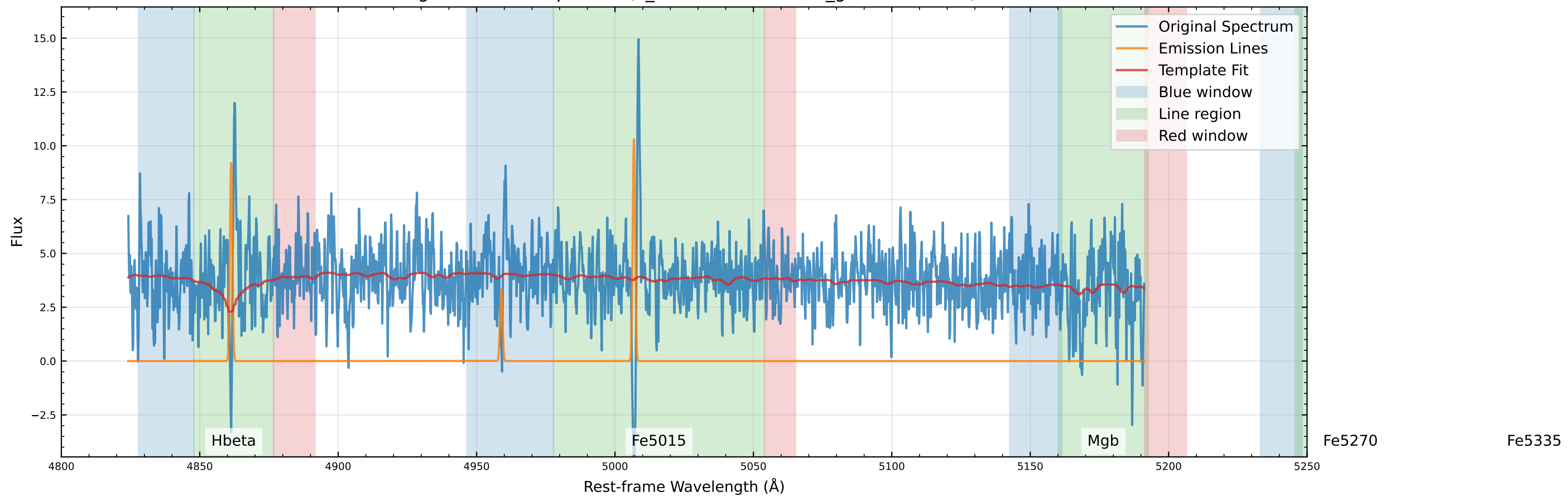
Original Data Comparison (v_star=111.1 km/s, v_gas=94.2 km/s)
